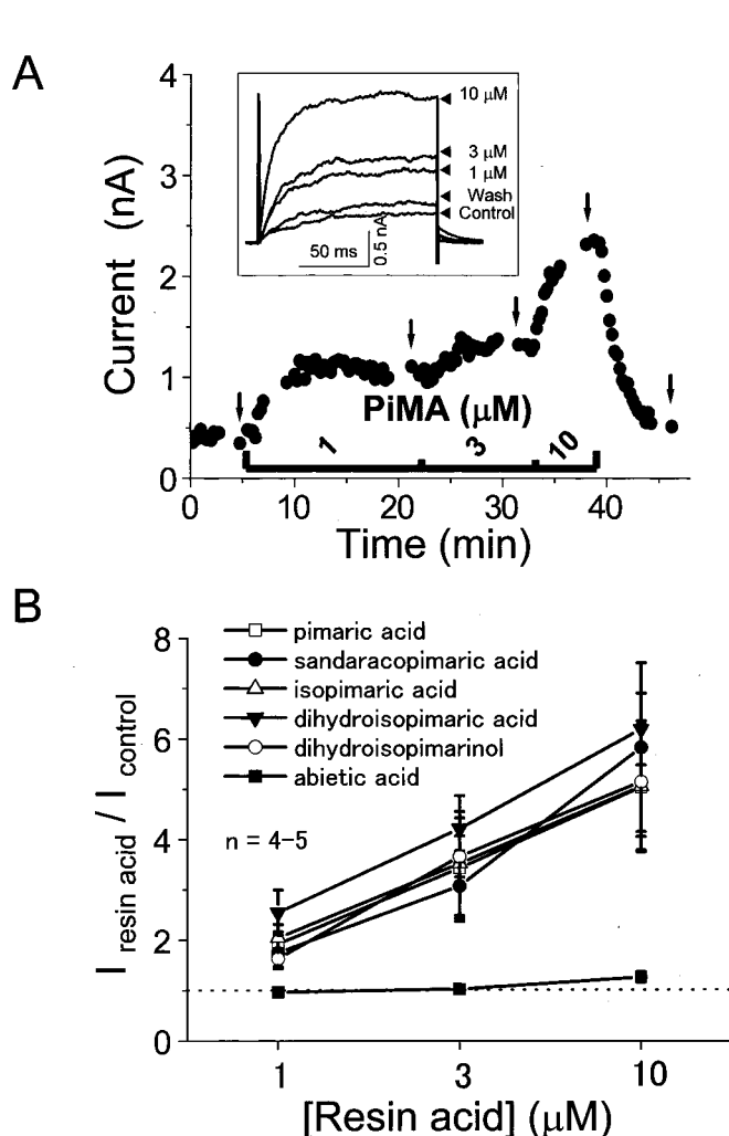
Fig. 3. Effects of PiMA and related compounds on macroscopic membrane currents in HEKKBK \alpha 1 cell. A , single HEKKBK \alpha 1 cell was depolarized from -60 to +30 mV for 150 ms under whole-cell voltage clamp. PiMA was applied cumulatively in a concentration range of 1 and 10 \mu\text{M} . Original current recordings at different concentrations were superimposed and shown in the inset. The peak outward current amplitude at +30 mV was measured and plotted against time. The original traces were obtained at the time indicated by vertical arrows in the time course. B , the concentration-response relationships for several resin acids. Effects of PiMA ( \square ), sandaracopimaric acid ( \bullet ), isopimaric acid ( \triangle ), dihydroisopimaric acid ( \nabla ), dihydroisopimarinol ( \circ ), and abietic acid ( \blacksquare ) were examined in experiments identical to that shown in A for PiMA. The relative amplitude of peak outward current at +30 mV in the presence of test compounds ( I_{\text{resin acid}}/I_{\text{control}} ) was determined taking the amplitude in the absence of them as unity (dotted line). Symbols and vertical bars show mean values and S.E.M., respectively; there were 4 to 5 experiments for each compound.
