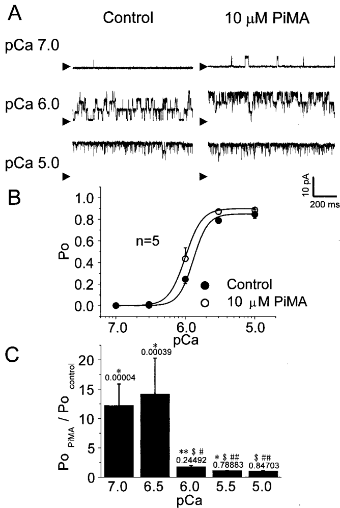
Fig. 8. Effects of PiMA on \text{Ca}^{2+} dependence of BK \alpha . A, single-channel currents of BK \alpha were recorded in inside-out patch configuration at +40 mV in asymmetrical \text{K}^+ conditions (5.9 and 140 mM \text{K}^+ ). Recordings were obtained at pCa 7.0, 6.0, and 5.0 in the absence and presence of 10 \mu\text{M} PiMA. B, the relationships between P_o and pCa in the bathing solutions were obtained in the absence (●) and presence of 10 \mu\text{M} PiMA (○). Number of examples was five for each. The data were fitted with the Hill equation. The fitted lines correspond to the following values of K_d , Hill coefficient, and the constant; 5.88, 4.15, and 0.153 in the absence and 5.98, 3.65, and 0.102 in the presence of 10 \mu\text{M} PiMA, respectively. C, the relative increase in P_o by application of 10 \mu\text{M} PiMA was reevaluated from the data shown in B. The P_o in the presence of 10 \mu\text{M} PiMA ( P_o \text{ PiMA} ) versus in its absence was illustrated against pCa. The numbers on the columns are the mean P_o in the absence of PiMA. *, p < 0.05 ; **, p < 0.01 versus unity. $, p < 0.05 versus P_o \text{ PiMA} / P_o \text{ control} at pCa 7.0. #, p < 0.05 ; ##, p < 0.01 versus P_o \text{ PiMA} / P_o \text{ control} at pCa 6.5.
