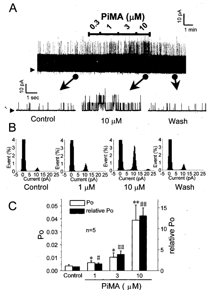
Fig. 5. Effects of PiMA on single BK \alpha channel currents recorded using the inside-out patch configuration. A, single channel currents were recorded at +40 mV in a patch from HEK293 cells using symmetrical 140 mM K + conditions. The Ca 2+ in the bathing solution was adjusted to pCa 7.0. PiMA was applied cumulatively at 0.3 to 10 \mu M. Selected parts of the trace indicated by arrows are shown as a faster time scale. B, amplitude histograms in the control, in the presence of 1 or 10 \mu M PiMA and after washout obtained from the recording shown in A. The ordinate expresses the relative time (%) spent at the corresponding amplitude in each bin (1 pA). C, summarized data demonstrating the relationship between concentrations of PiMA and open probability ( P_o ) of BK \alpha obtained from experiments shown in A. P_o was calculated from the histogram shown in B as the relative time spent at open state, based on the total number of BK \alpha channels in patches, which was determined by elevating Ca 2+ concentration to 4.0 (□). Only the data from patches including less than 5 channels were analyzed. The relative P_o is obtained taking the P_o in the absence of PiMA as unity (■); there were 6 examples. * and **, p < 0.05 and p < 0.01 versus control.
