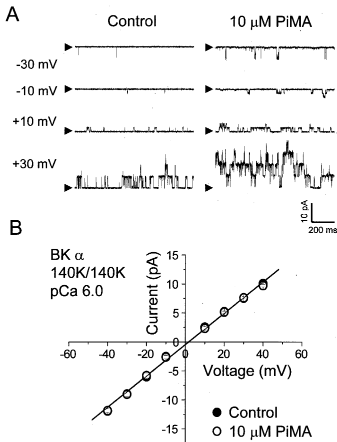
Fig. 6. Effects of PiMA on single-channel conductance of BK \alpha . A, single-channel currents of BK \alpha in inside-out patches were recorded at several potentials in the absence and presence of 10 \mu\text{M} PiMA. All conditions except applied potentials were the same as shown in Fig. 4. B, the current-voltage relationships obtained from the measurements shown in A. The relations in the absence (●) and presence of 10 \mu\text{M} PiMA (○) were fitted to linear lines, and the single channel conductance was determined from the slope. The number of observations was seven for each in the absence and presence of PiMA.
