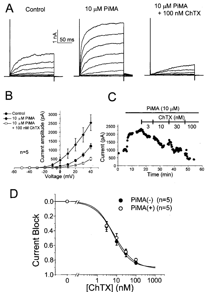
Fig. 4. Effects of PiMA on the blockade of macroscopic currents by charybdotoxin (ChTX) in HEKKBK \alpha 1 cell. A , each single HEKKBK \alpha 1 cell was depolarized from -60 mV by 10 mV step for 150 ms under whole-cell voltage clamp. Application of 10 \mu\text{M} PiMA and then 100 nM ChTX enhanced and then markedly reduced outward currents, respectively. B , the current-voltage relationships were obtained in the control ( \bullet ), in the presence of PiMA ( \blacklozenge ), and after the further addition of 100 nM ChTX ( \square ) in experiments such as illustrated in A ; five examples. C , the time course of effects of PiMA and ChTX on peak outward currents elicited by depolarizations from -60 to +40 mV applied once every 15 s. ChTX was added cumulatively at concentrations of 3 , 10 , 30 , and 100 nM in the presence 10 \mu\text{M} PiMA. D , the relationship between ChTX and the block of outward currents obtained from experiments shown in C . The relative amount of block was defined as the relative amplitude of the current reduced by ChTX versus the amplitude before addition of ChTX in each cell in the absence ( \bullet ) or presence ( \circ ) of 10 \mu\text{M} PiMA ( n = 5 for each). The data were fitted with Hill equation modified for the concentration-block relationship. The fitted lines were drawn based on the following values of K_d , Hill coefficient and the constant; 7.66 , 0.847 , and 0.771 in the control and 6.72 , 0.982 , and 0.0965 in the presence of 10 \mu\text{M} PiMA, respectively.
