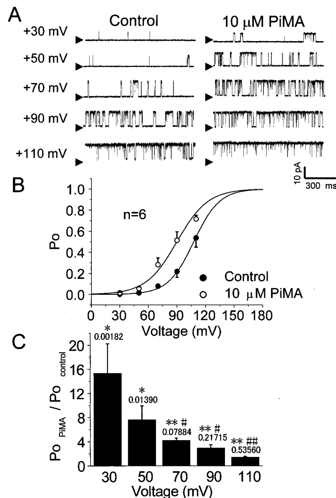
Fig. 7. Effects of PiMA on voltage dependence of BK \alpha . A, single-channel currents of BK \alpha were recorded in inside-out patch configuration at pCa 7.0 in symmetrical 140 mM \text{K}^+ conditions. Recordings were obtained at several test potentials in the range, +30 and +110 mV, in the absence and presence of 10 \mu\text{M} PiMA. B, the relationships between P_o and test potentials were obtained in the absence (●) and presence of 10 \mu\text{M} PiMA (○). Number of examples was six for each. The data were fitted using the Boltzmann relationship. The fitted lines are based on the following values of V_{1/2} and slope factor; 106.0 and 13.3 mV, in the absence and 85.6 and 11.8 mV in the presence of 10 \mu\text{M} PiMA, respectively. C, the relative increase in P_o after application of 10 \mu\text{M} PiMA was reevaluated from the data shown in B. The relative P_o in the presence of 10 \mu\text{M} PiMA ( P_{o \text{ PiMA}} ) versus in its absence ( P_{o \text{ control}} ) was illustrated against the test potentials. The numbers on the columns are the mean P_o in the absence of PiMA. *, p < 0.05 ; **, p < 0.01 versus unity. #, p < 0.05 ; ##, p < 0.01 versus P_{o \text{ PiMA}}/P_{o \text{ control}} at +30 mV.
