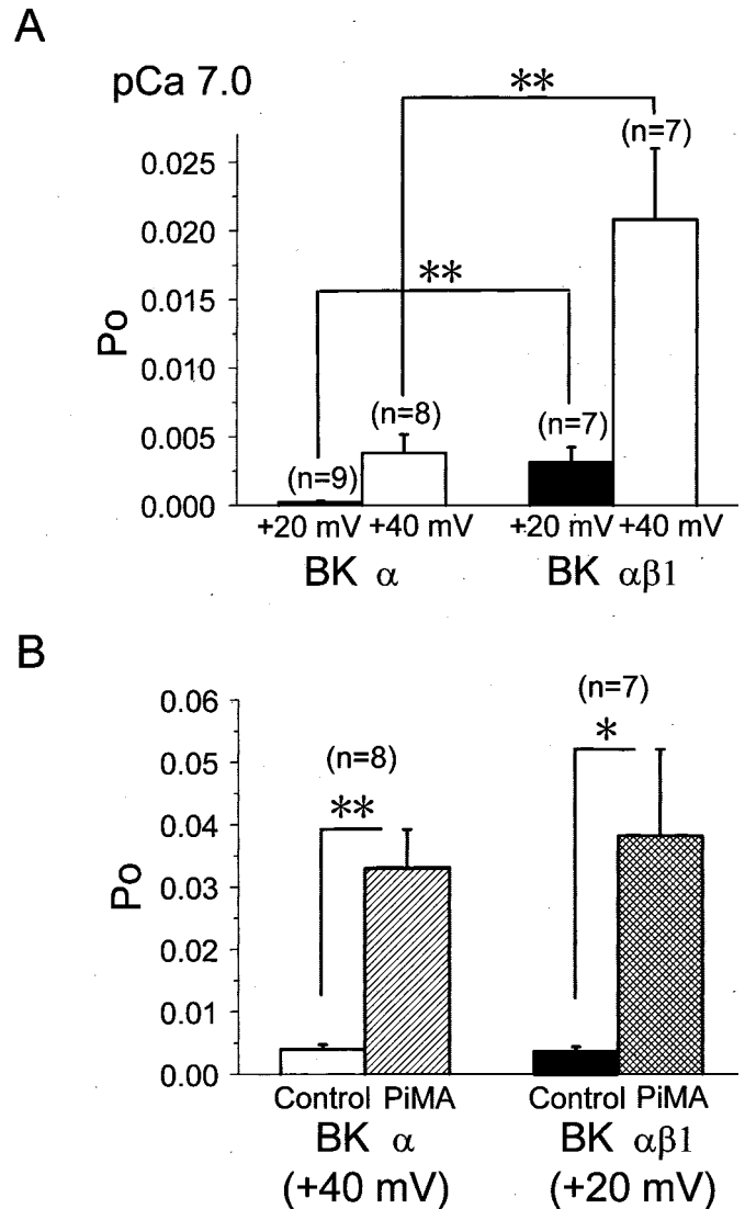
Fig. 9. Comparison of effects of PiMA on single-channel currents caused by BK \alpha or BK \alpha 1. A, P_o was obtained from inside-out patches recording from HEKBK \alpha and HEKBK \alpha 1 under following conditions: pCa 7.0, the holding potential of +20 or +40 mV and symmetrical 140 mM \text{K}^+ solutions. The P_o at +20 and +40 mV in BK \alpha 1 were significantly higher than that in BK \alpha (**, p < 0.01 ). Number of examples was six for each. B, the effect of 10 \mu\text{M} PiMA on P_o of BK \alpha 1 was compared with that of BK \alpha . The P_o of BK \alpha and BK \alpha 1 in the absence of PiMA were 0.00346 \pm 0.00079 at +20 mV and 0.00382 \pm 0.00104 at +40 mV, respectively ( p > 0.05 ). The P_o were increased to 0.03297 \pm 0.00629 and 0.03061 \pm 0.01237 in BK \alpha and BK \alpha 1 by application of 10 \mu\text{M} PiMA, respectively. Number of examples was six for each. *, p < 0.05 ; **, p < 0.01 versus the corresponding control.
