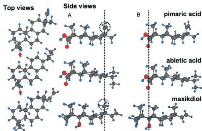
Fig. 10. Stereoscopic structures of pimaric acid, abietic acid, and maxikdiol.
