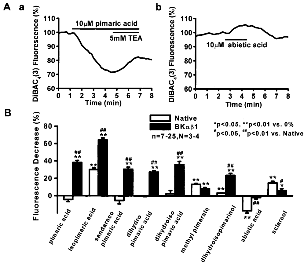
Fig. 2. Measurements of DiBAC 4 (3) fluorescence in HEK293 cells heterologously expressing BK channel \alpha and \beta 1 subunits (HEK \alpha BK \beta 1) and effects of nine compounds shown in Fig. 1. A, fluorescence intensity of DiBAC 4 (3) was measured from clusters of HEK \alpha BK \beta 1 in the continuous presence of 50 or 100 nM dye after loading for 20 min. PiMA (a) and abietic acid (b) were applied at the concentration of 10 \mu M. Each cluster included 10 to 30 cells. The fluorescence intensity measured at 1 min before the application of test compounds was taken as 100%. The perfusion solutions contained 0.1% DMSO throughout. When a test compound decreased fluorescence, 5 mM TEA was added (a). B, Summarized data demonstrating the relative decrease in fluorescence intensity of DiBAC 4 (3) after application of nine test compounds. Each of these compounds was also applied to native HEK293 cells as the control. \square , relative decrease in fluorescence intensity in native HEK; \blacksquare , relative decrease in fluorescence intensity in HEK \alpha BK \beta 1. Mean values and S.E.M. are depicted as columns and vertical bars. Data were accumulated from 7 to 25 clusters ( n ) from 3 to 4 separate culture dishes ( N ) for each column. **, p < 0.01 versus 0% in each column. #, p < 0.05 ; ##, p < 0.01 versus native HEK in a pair of each compound.
