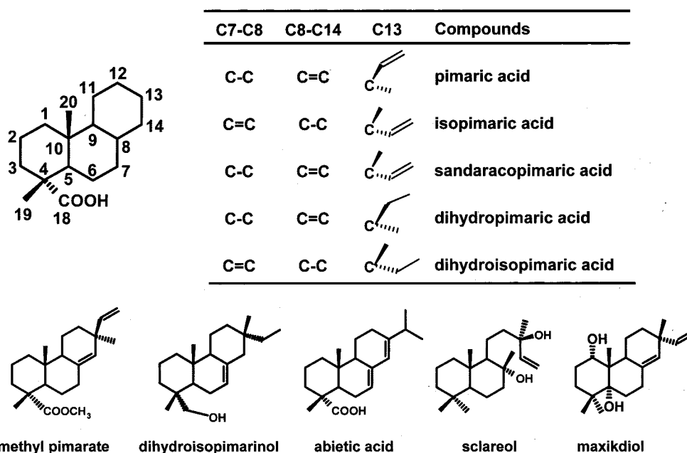
Fig. 1. Chemical structures of compounds selected for testing; resin acids contained in pine rosin and their derivatives and maxikdiol.
